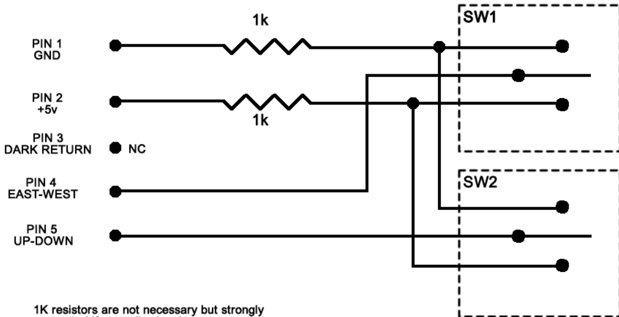
Heliotrack Dual Axis Remote Control *Without Dark Return Disable
